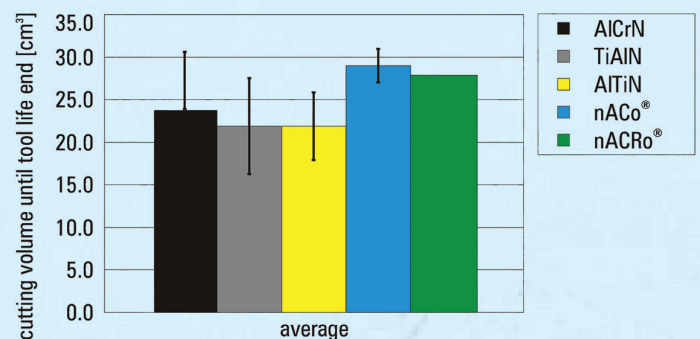
Tool Life Comparison in Inconel 718
